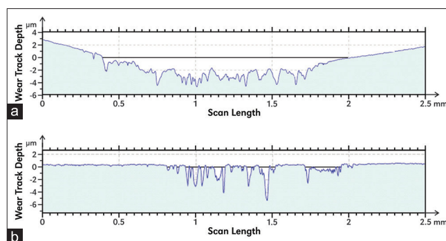
Figure 2: Wear tracks of Opal seal (OS) (a) and Pro Seal (PS) (b) traced by a contact profilometer. Average volume of wear of OS is significantly greater than that of PS ( P < 0.01 )
