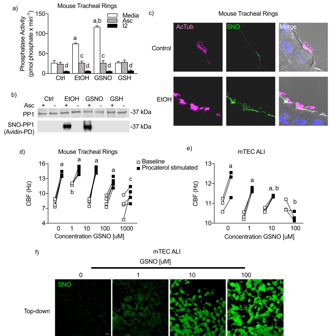
Figure 3. GSNO recapitulates AICD in mouse tracheal rings. (a) GSNO (4 h \times 1 mM) and alcohol (EtOH; 100 mM \times 10 days) increase PP1 activity in mouse tracheal rings, which is reversed by ascorbate (10 min \times 30 \mu M). Data are representative of the mean of 3–6 tracheal rings from 4 mice. a p < 0.05 compared to media control. b p < 0.005 compared to EtOH. c p < 0.05 compared to media within group. d p < 0.05 compared to Asc within group. (b) GSNO and EtOH increase biotin switch detection of PP1 in mouse tracheal rings. The absence of Asc is a negative control for the biotin switch assay. (c) In vitro EtOH increases cilia S-nitrosation in mouse tracheal rings. Acetylated tubulin (AcTub) - pink; Avidin-fluorescein (SNO) - green (d) GSNO (4 h) blocks procaterol (1 h \times 10 nM) stimulation in mouse tracheal rings. a p < 0.0001 compared to baseline of the same condition. b p < 0.001 compared to control baseline. c p < 0.01 compared to control stimulated. Data are representative of 3–4 tracheal rings from 4–5 mice per condition. (e) GSNO (4 h) blocks procaterol stimulation in cultured mouse tracheal epithelial cells. a p < 0.001 compared to baseline of the same condition. b p < 0.001 compared to control stimulated. n = 13 –24 cultures per group. (f) GSNO (4 h) increases S-nitrosation in mouse tracheal epithelial cells. Top : Looking down on ALI culture. Avidin-fluorescein (SNO) – green.
