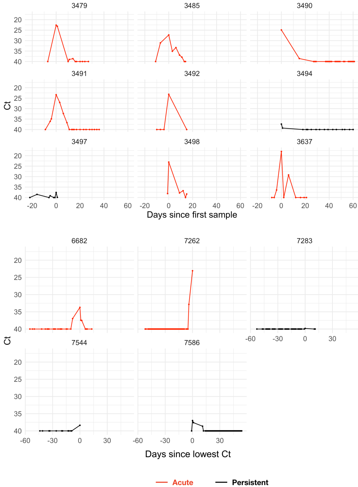
S5 Fig. Observed Ct values from the study participants (4/4). Points depict observed Ct values, which are connected with lines to better visualize trends. Individuals with presumed acute infections are marked in red. All others are in black. Underlying data are available at https://github.com/gradlab/CtTrajectories/tree/main/data 10
